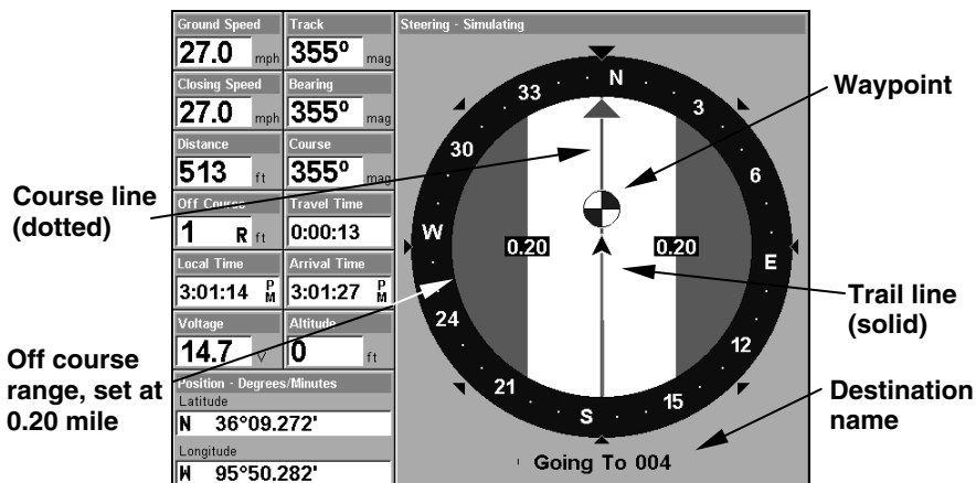
Navigation Page, navigating toward waypoint 004 and leaving a trail.
